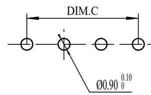
PCB LAYOUT
