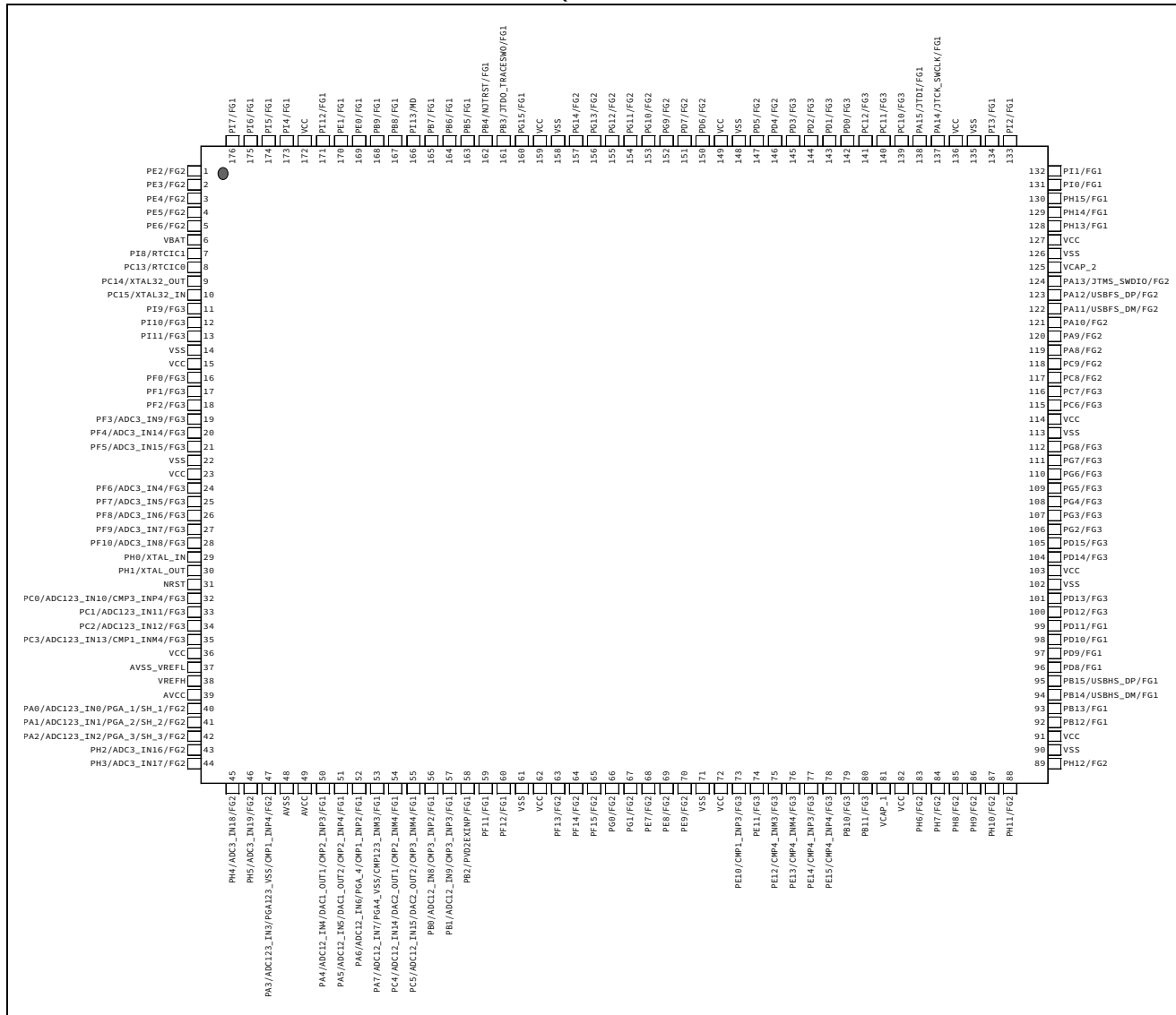
LQFP176
