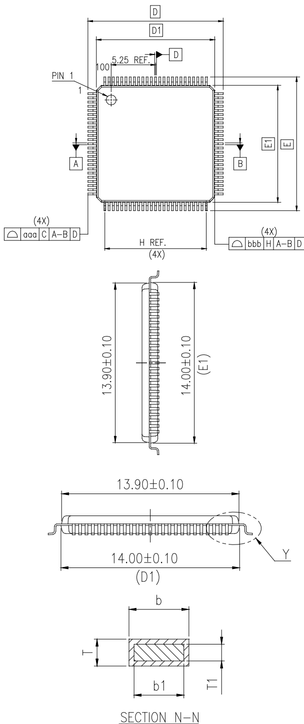
DIMENSION LIST ( FOOTPRINT: 2.00)
