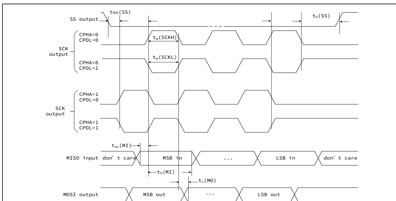
图 3-12 SPI timing diagram -master mode
