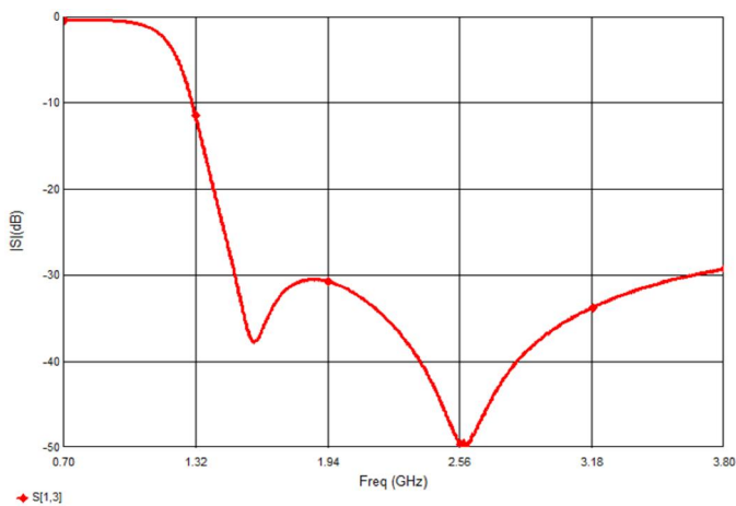
Low-Band Attenuation
