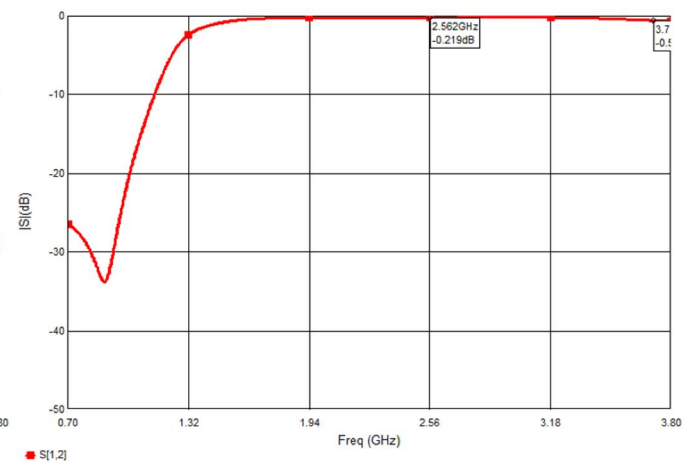
High-Band Attenuation
