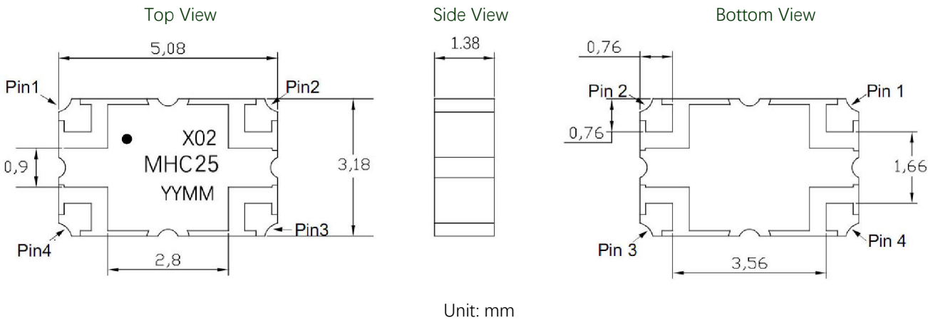
Figure 2. MHC25X02 Outline Drawing
