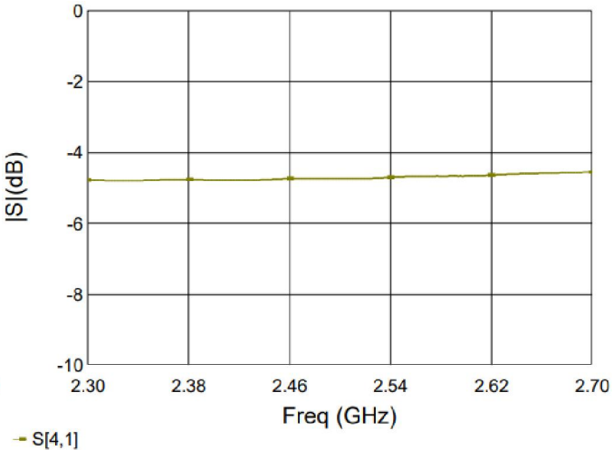
Figure 4. MHC25X02 Transmission
