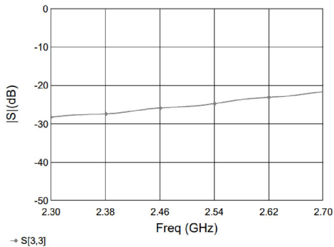
Figure 7. MHC25X02 Return Loss (S33)
