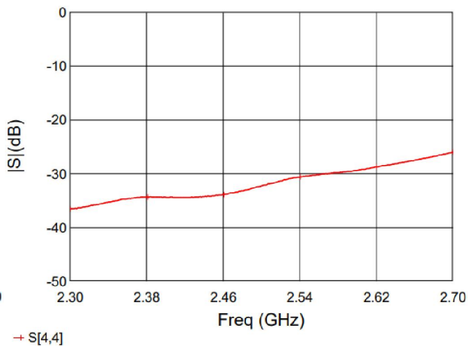
Figure 8. MHC25X02 Return Loss (S44)
