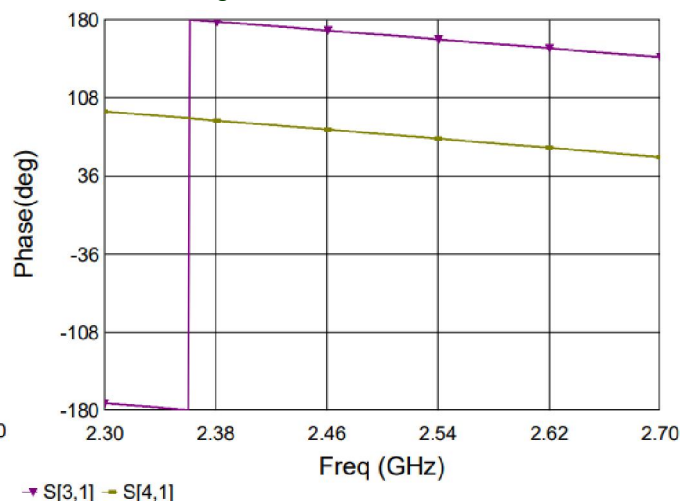
Figure 10. MHC25X02 Phase
