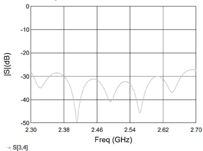
Figure 9. MHC25X02 Isolation
