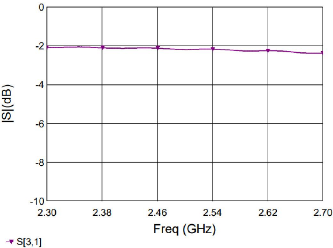
Figure 3. MHC25X02 Coupling
