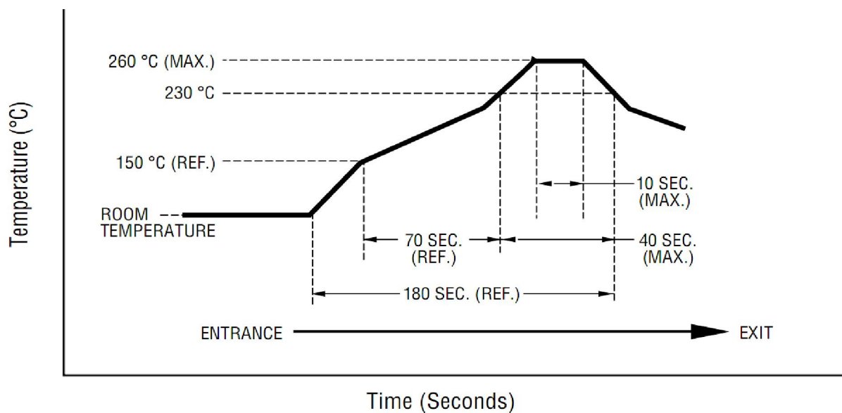
Figure 10. MBF1565D33 Recommended Reflow Solder Profile
