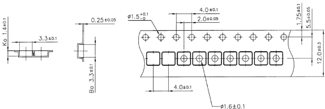
Figure 9. MBF1565D33 Packaging Specifications
