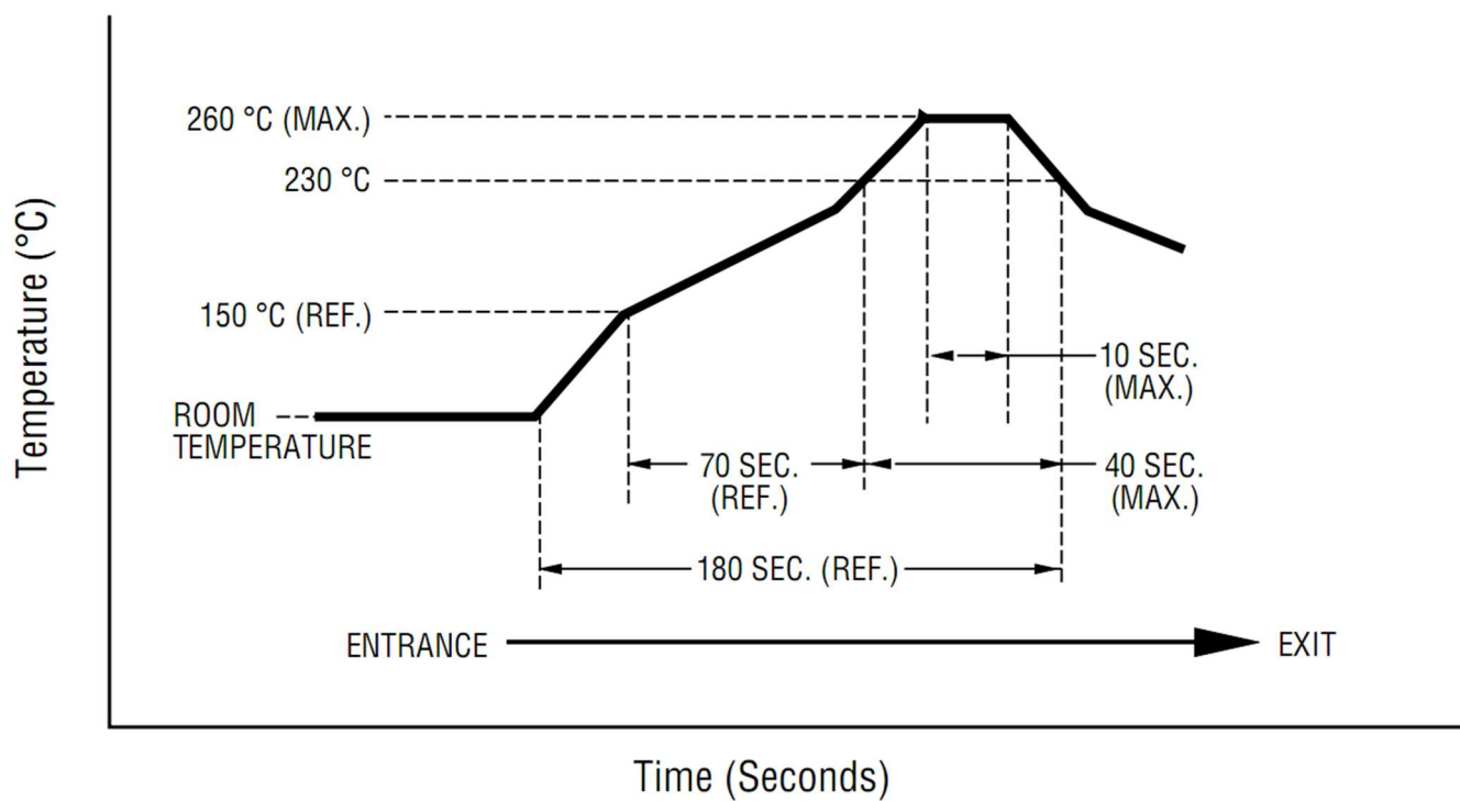
Figure 12. MHC0600L03 Thermal Reflow Profile
