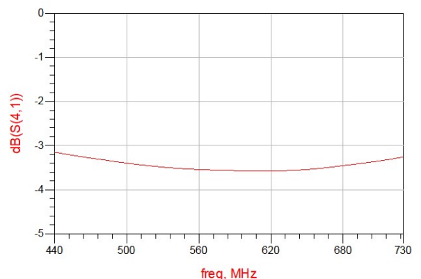
Figure 4. MHC0600L03 Transmission
