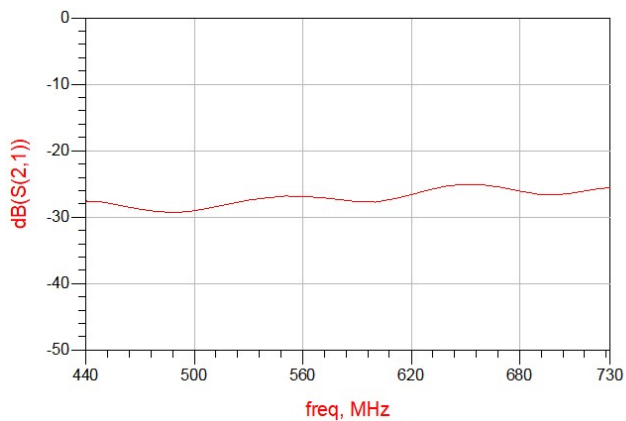
Figure 9. MHC0600L03 Isolation
