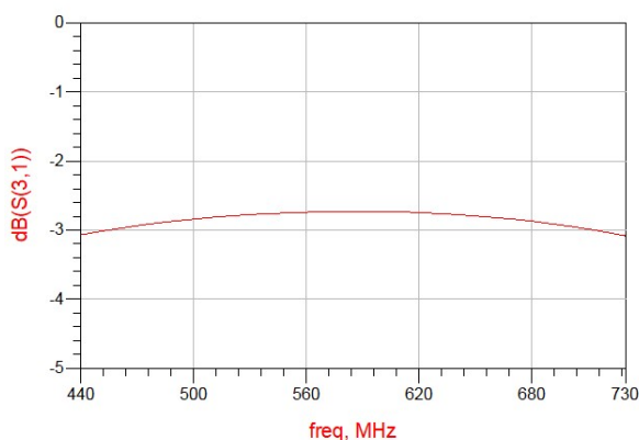
Figure 3. MHC0600L03 Coupling
