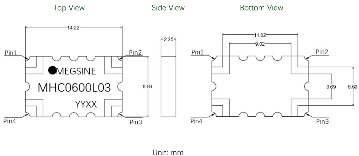
Figure 2. MHC0600L03 Outline Drawing
