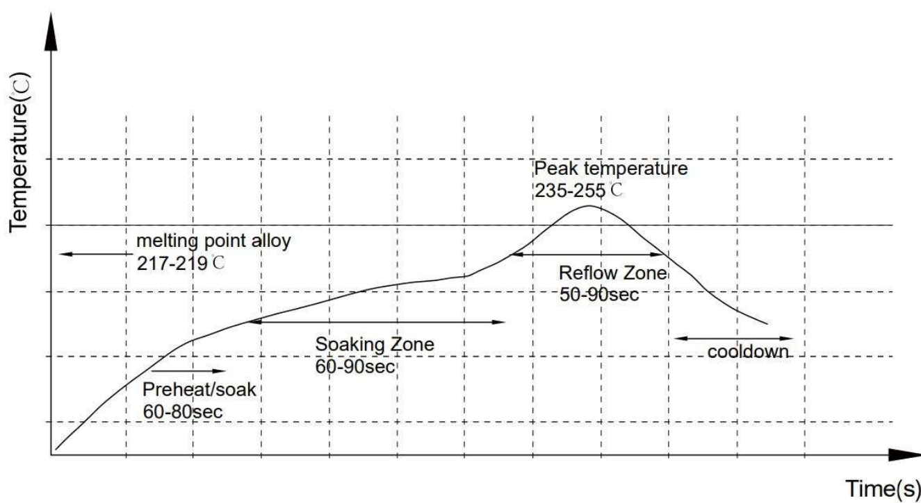
Figure 12. Thermal Reflow Profile
