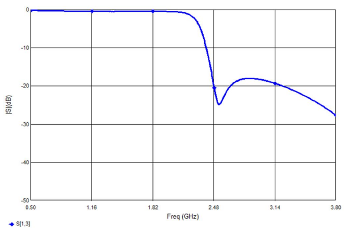
Low-Band Attenuation
