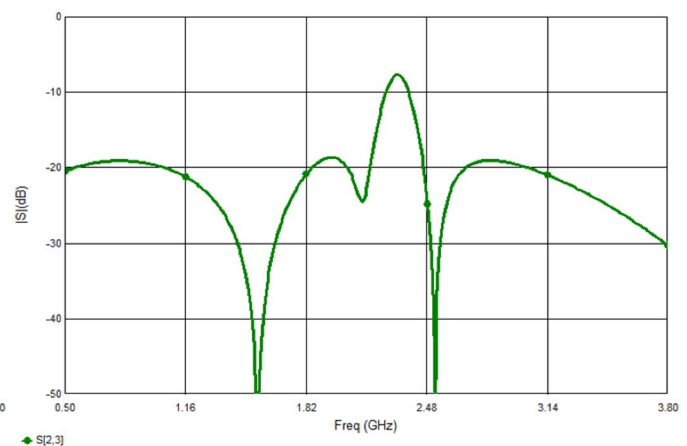
Common Isolation
