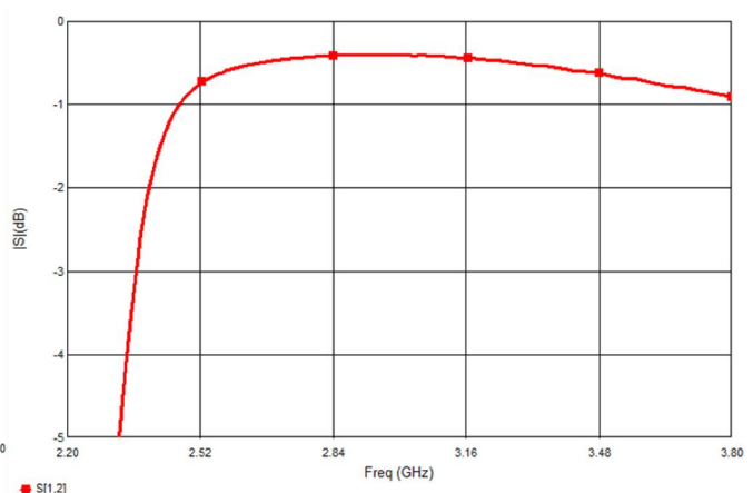
High-Band Insertion
