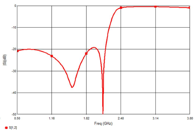
High-Band Attenuation
