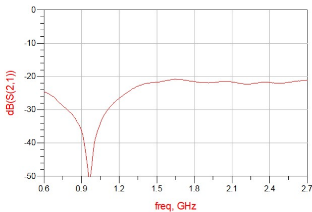
Figure 9. MHC0627L03 Isolation
