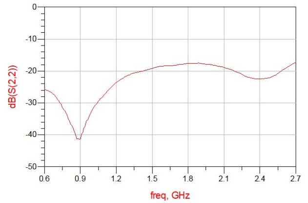
Figure 6. MHC0627L03 Return Loss (S22)
