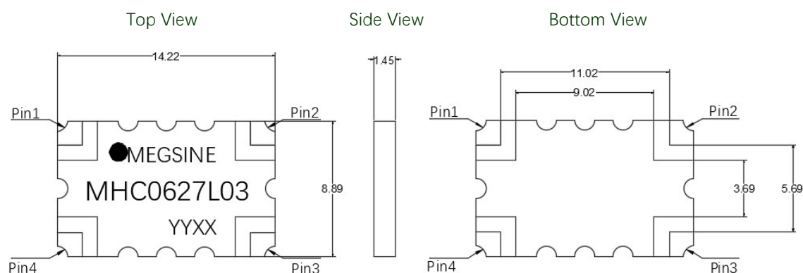
Figure 2. MHC0627L03 Outline Drawing
