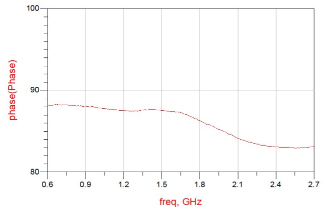
Figure 10. MHC0627L03 Phase
