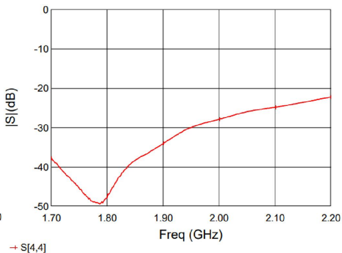
Figure 8. MHC21X02 Return Loss (S44)
