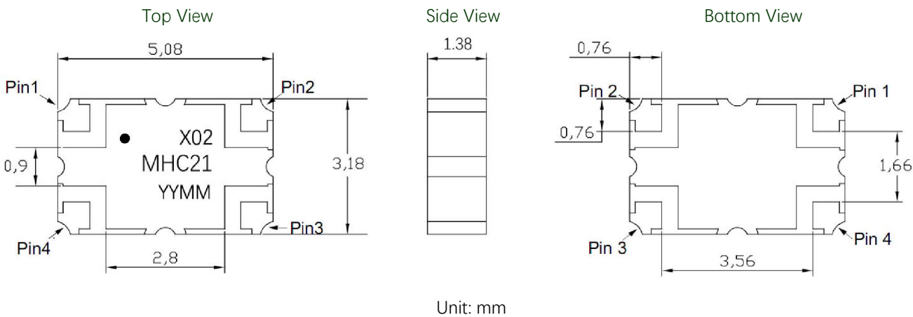
Figure 2. MHC21X02 Outline Drawing
