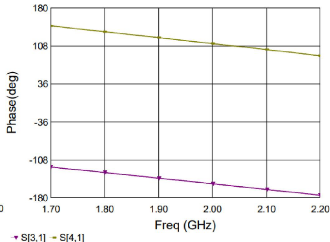
Figure 10. MHC21X02 Phase
