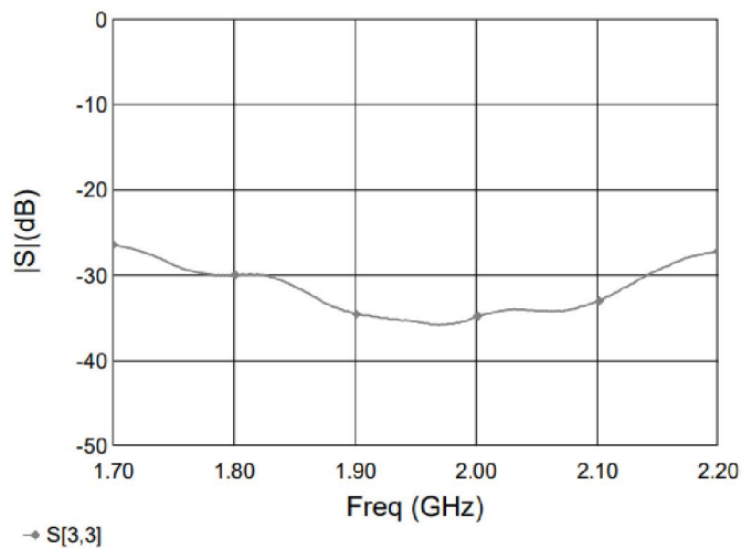
Figure 7. MHC21X02 Return Loss (S33)
