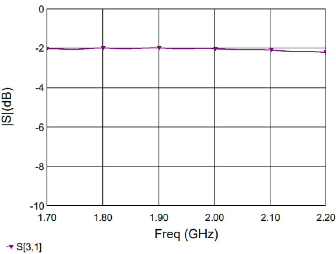
Figure 3. MHC21X02 Coupling
