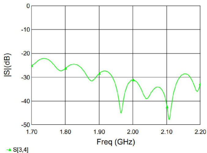
Figure 9. MHC21X02 Isolation
