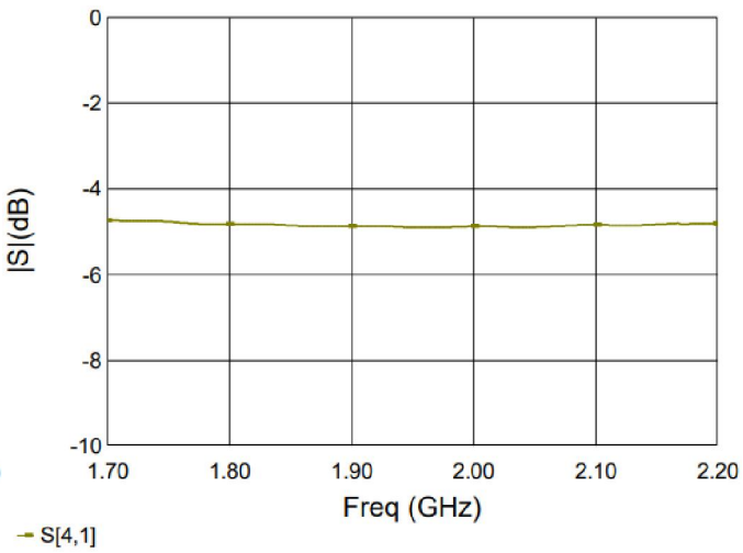
Figure 4. MHC21X02 Transmission
