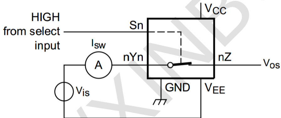
Figure 7. Test circuit for measuring OFF-state current
