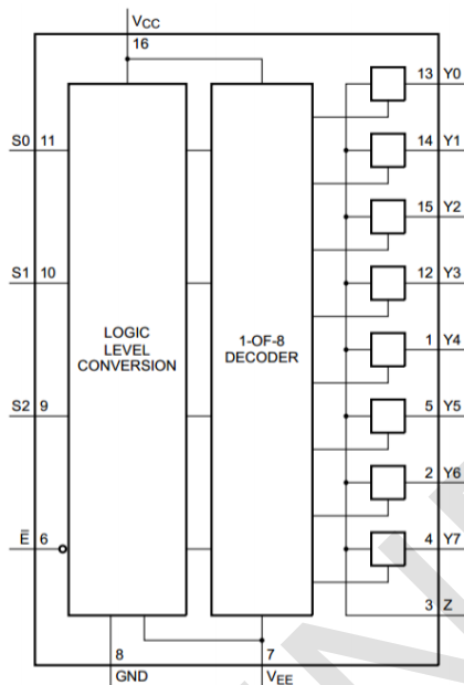
Figure 4. Functional diagram
