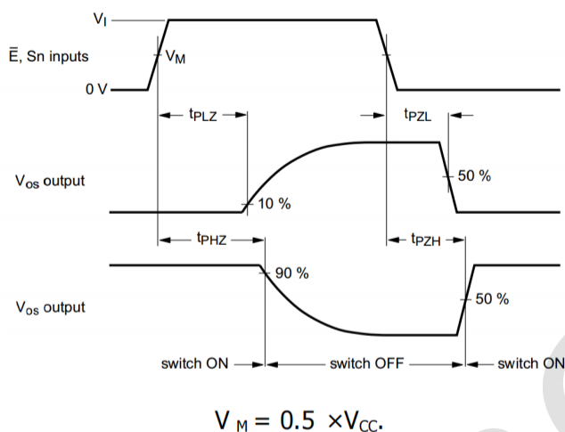
Figure 10. Turn-on and turn-off times
