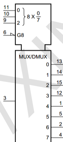
Figure 2. IEC logic symbol
