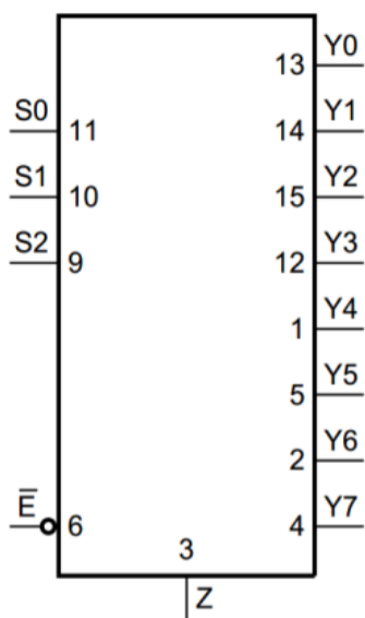
Figure 1. Logic symbol
