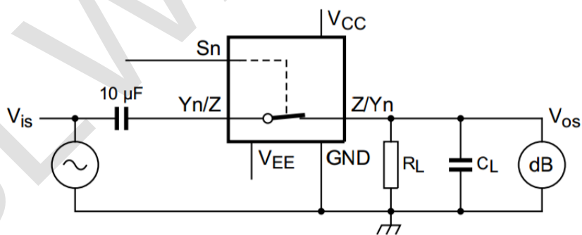
Figure 12. Test circuit for measuring sine-wave distortion
