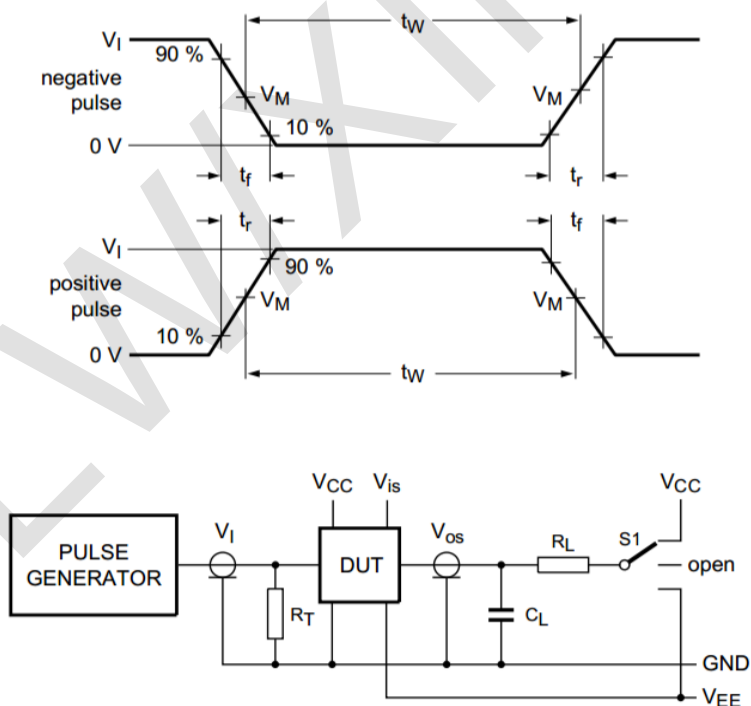
Figure 11. Test circuit for measuring switching times
