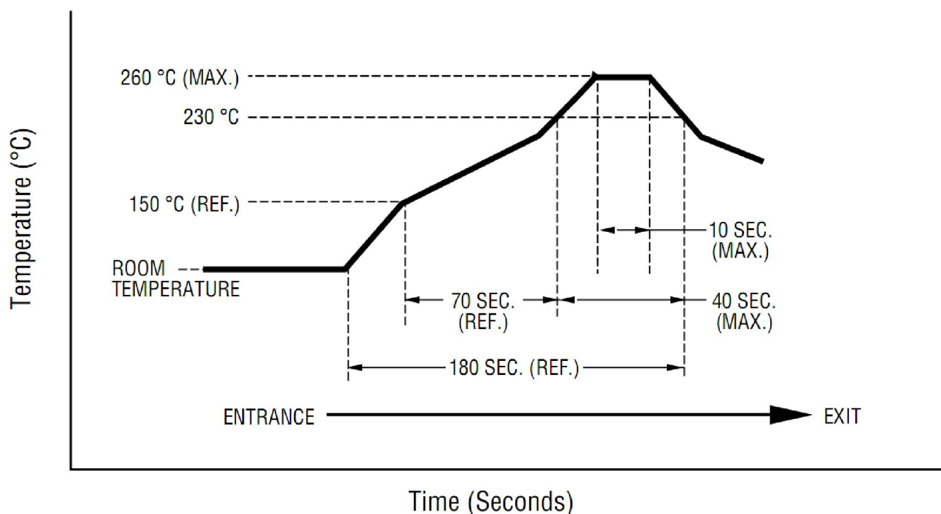
Figure 7. MHC21X03 Thermal Reflow Profile
