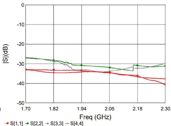
Figure 4. MHC21X03 Return Loss
