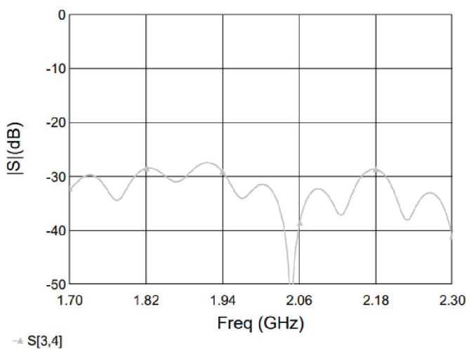
Figure 5. MHC21X03 Isolation
