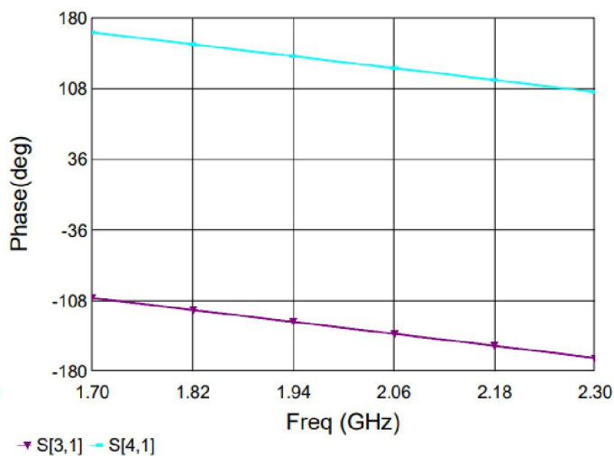
Figure 6. MHC21X03 Phase
