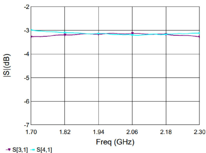
Figure 3. MHC21X03 Coupling & Transmission
