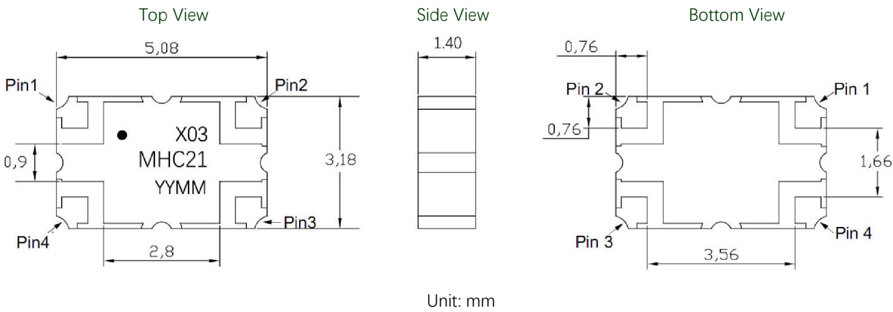
Figure 2. MHC21X03 Outline Drawing
