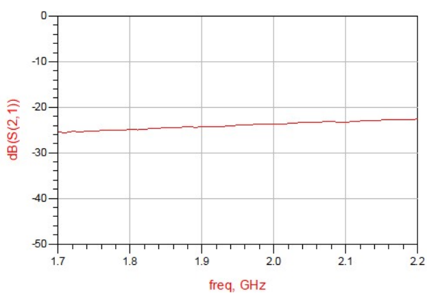
Figure 9. MHC2100L03 Isolation
