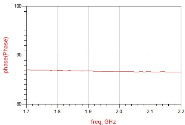
Figure 10. MHC2100L03 Phase
