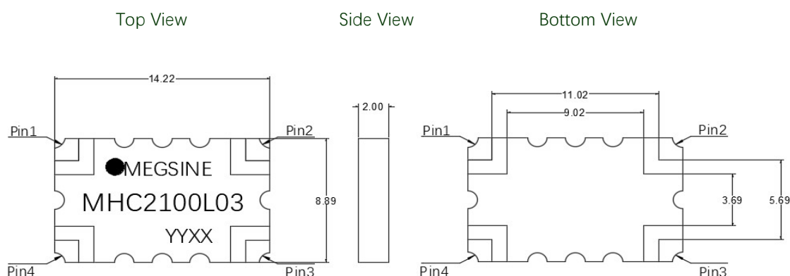
Figure 2. MHC2100L03 Outline Drawing
