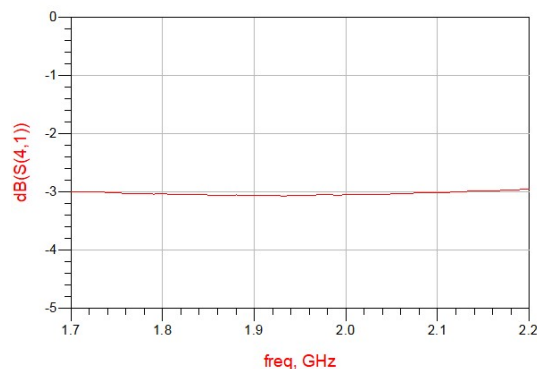
Figure 4. MHC2100L03 Transmission
