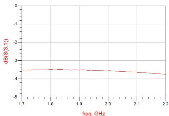
Figure 3. MHC2100L03 Coupling
