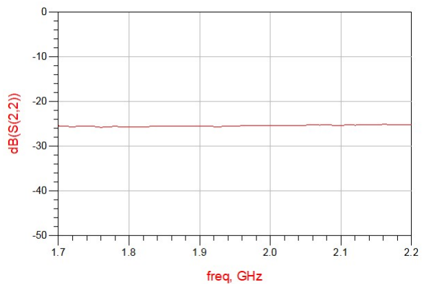
Figure 6. MHC2100L03 Return Loss (S22)
