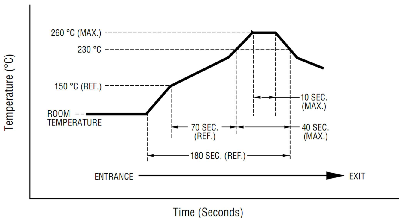
Figure 12. MHC2100L03 Thermal Reflow Profile
