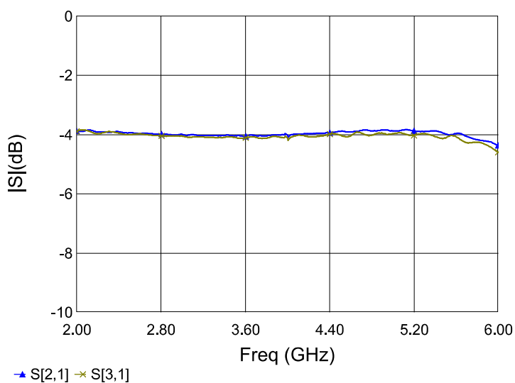
Figure 3. MPD2060W2 Insertion Loss
