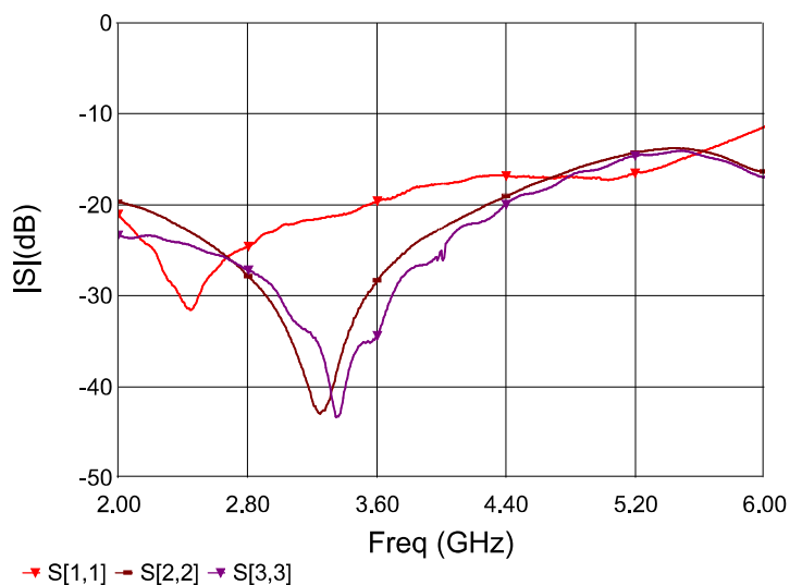
Figure 4. MPD2060W2 Return Loss
