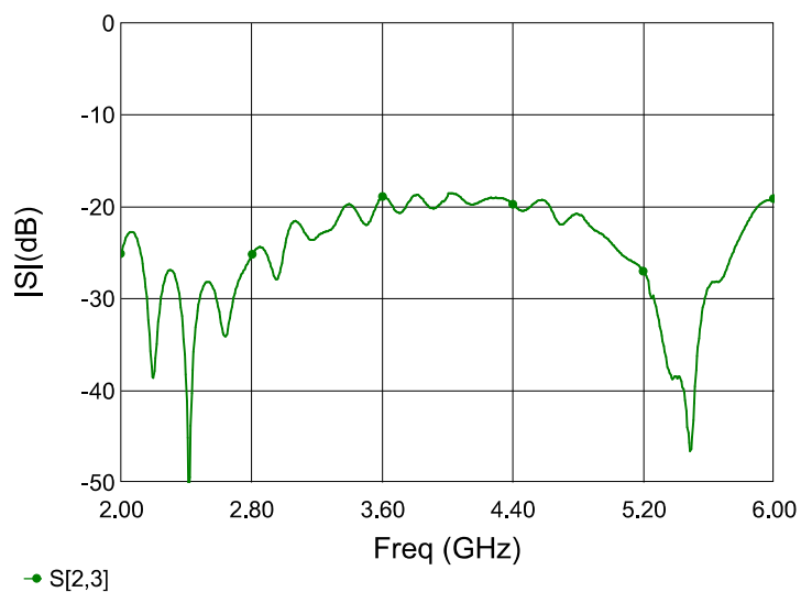
Figure 5. MPD2060W2 Isolation
