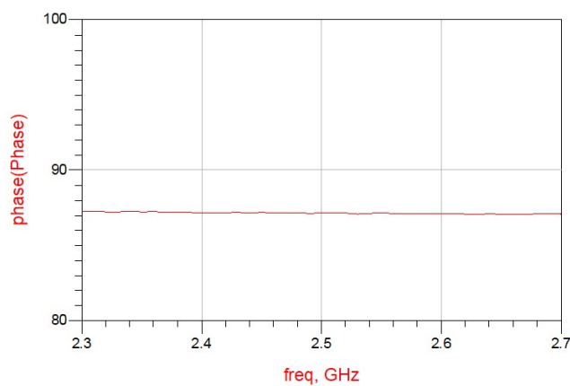
Figure 10. MHC2500L03 Phase
