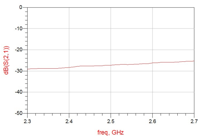
Figure 9. MHC2500L03 Isolation
