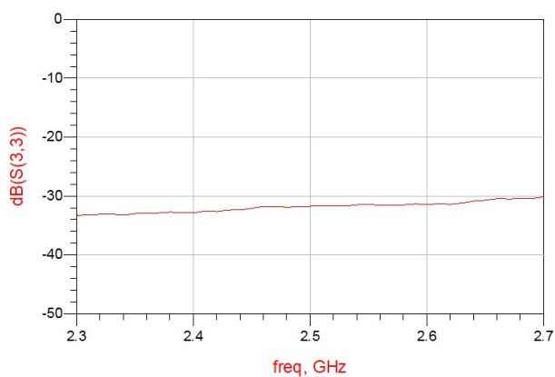
Figure 7. MHC2500L03 Return Loss (S33)
