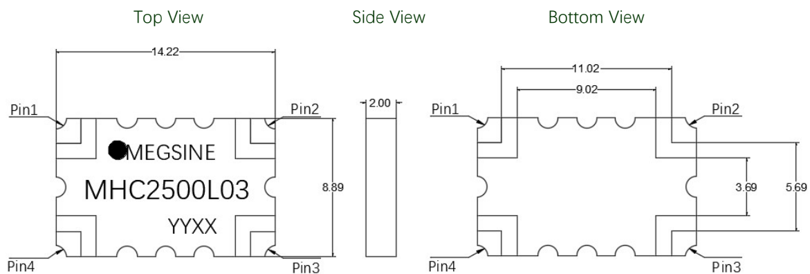
Figure 2. MHC2500L03 Outline Drawing
