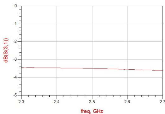
Figure 3. MHC2500L03 Coupling
