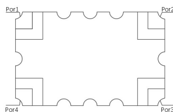
Figure 1. MHC2500L03 (Bottom View)
