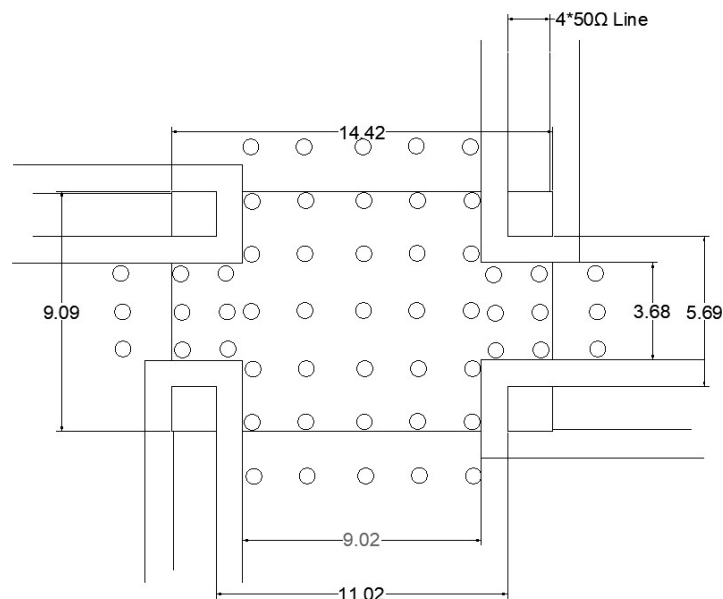
Figure 11. Recommended PCB Layout
