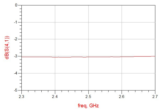
Figure 4. MHC2500L03 Transmission
