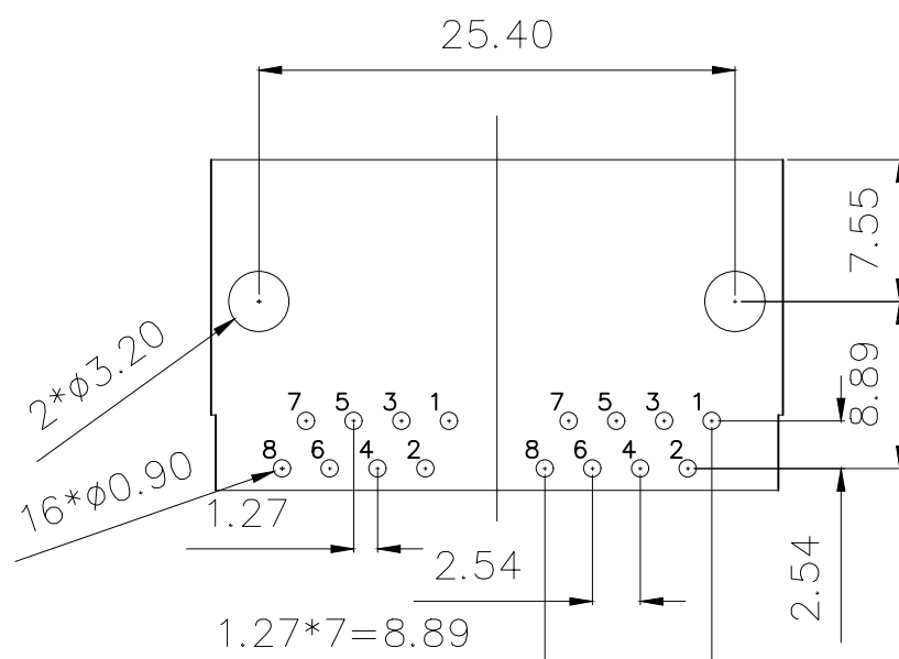
RECOMMENDED PCB LAYOUT TOP VIEW(TOL:±0.05)
