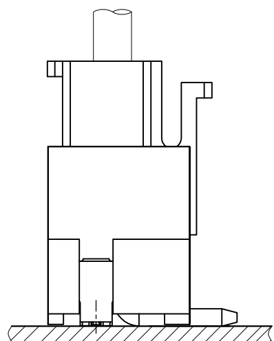
Assembly Layout
