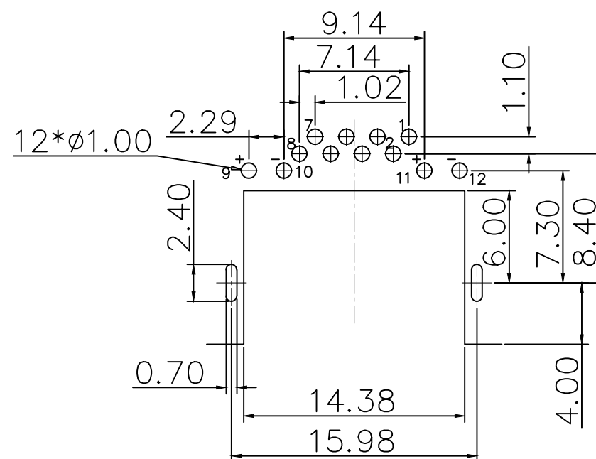
RECOMMENDED P.C.B LAYOUT TOP VIEW (COMPONENT SIDE)
