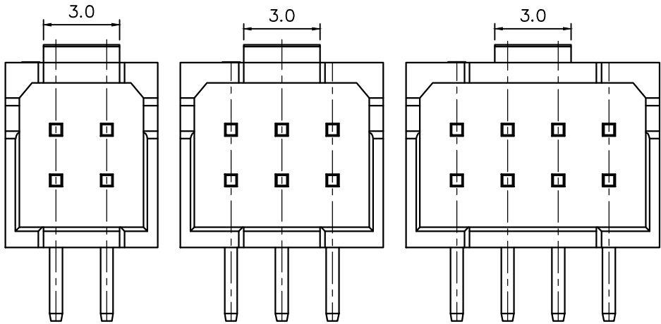
2~3P结构(2~3Pin Structure)
