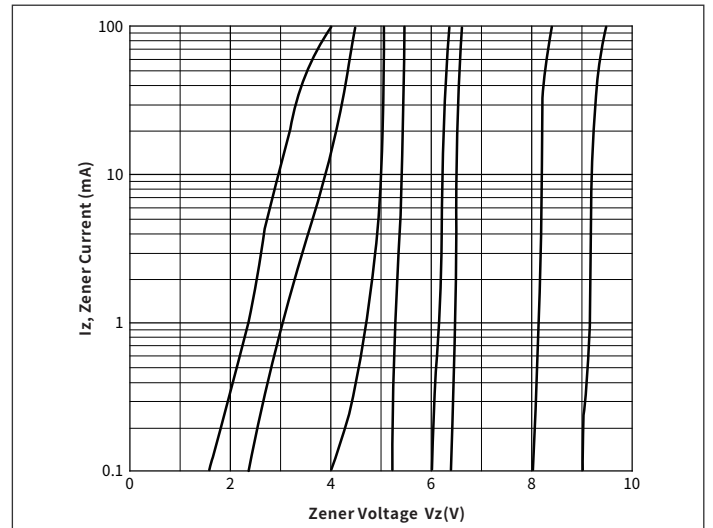
Fig.2 Zener Characteristics ( V_z 3.3V to 10V)
