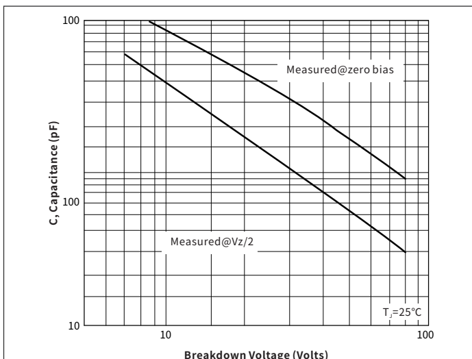
Fig.5 Typical Capacitance
