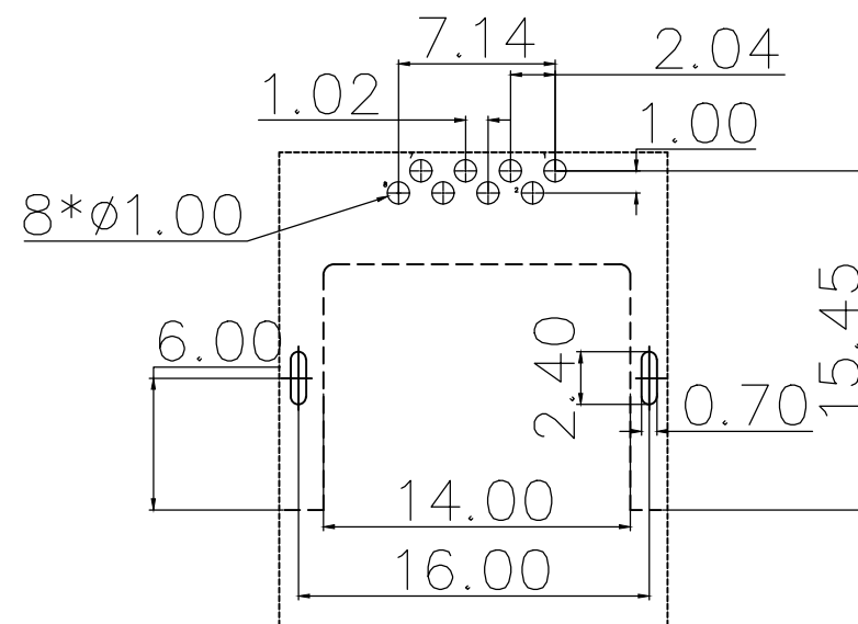
RECOMMENDED P.C.B LAYOUT TOP VIEW (COMPONENT SIDE)
