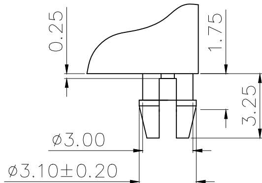
DETAIL "X" SCALE 2:1
