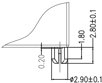
DETAIL "X" SCALE 2:1
