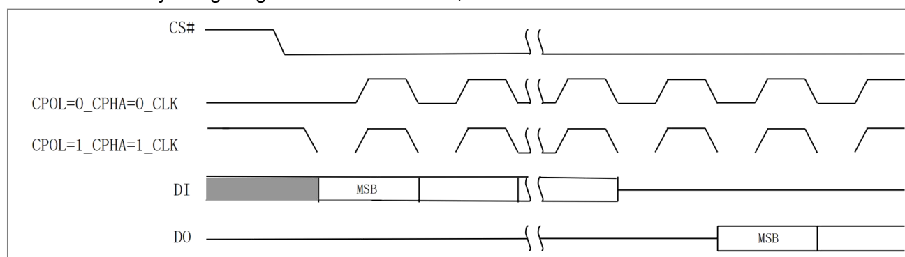
Figure 7.1 SPI Modes
