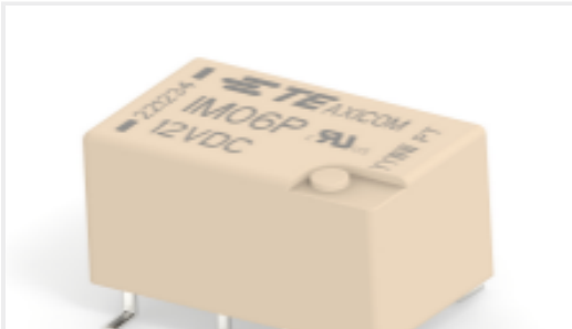
TE Part #5-1462039-6 IM06PGR=IM RELAY 140mW 12V
