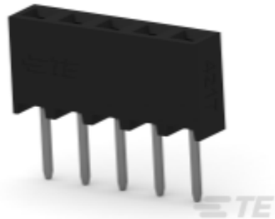
TE Part #2314876-5 5P,2MM,B-B,REC,SRVT,2.7,0.1AU,TB
