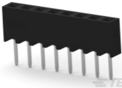
TE Part #2314876-8 8P,2MM,B-B,REC,SRVT,2.7,0.1AU,TB
