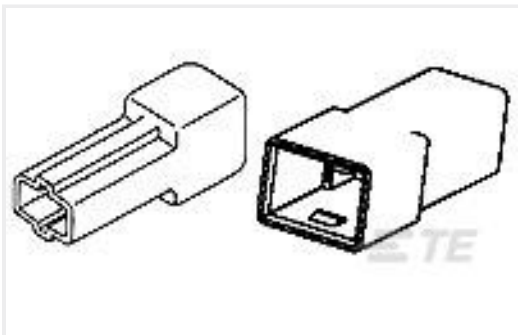
TE Part #880309-1 1 WAY FF 250 HOUSING TAB NYLON 6.6 NAT
