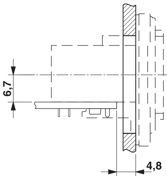
Dimensional drawing
