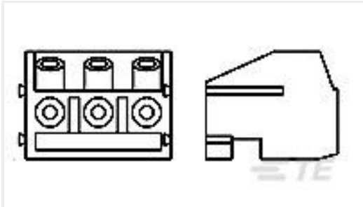
TE Part #1776263-4 4P TB Plug,w/interlock,90deg,5mm, Blue
