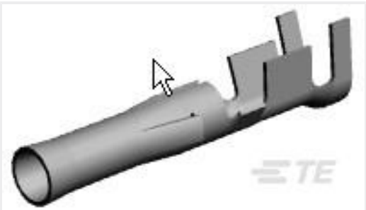
TE Part #350415-5 .093 COMM P&S SOK 20-14 AUBR
