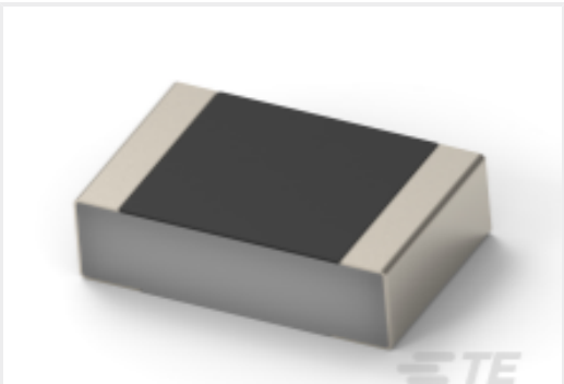
TE Part #3-2176453-1 CPF 0201 11K8 0.1% 25ppm 1K RL
