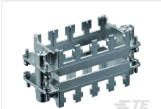
TE Part #T2070164001-000 H16BN-T4
