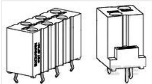
TE Part #1811957-1 ASY,SCRLESS WIRE CONN,VERT,2P
