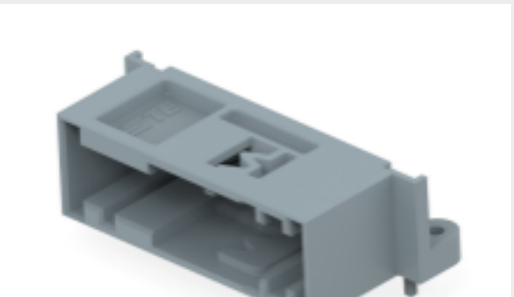
TE Part #2344642-1 32POS,TAB0.63X0.63,HDR ASSY, 90DEG,SLDR
