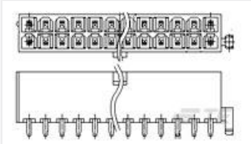
TE Part #3-1775099-2 ATX PWR CONN 1 BDLK 8 POS
