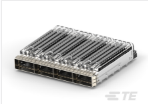
TE Part #5-2170790-4 CAGE ASSY, 1X4, QSFP28, SPRING, HS, LP
