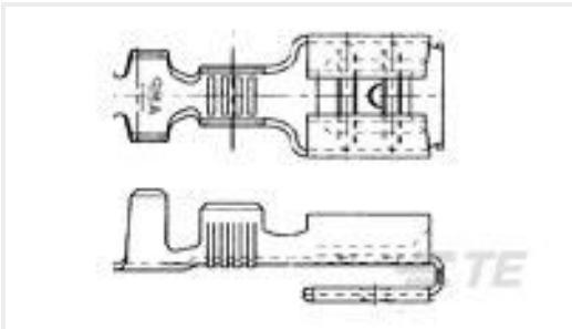
TE Part #160739-4 250 FASTON,PIGGYBACK REC.,18-14 AWG,TPPB
