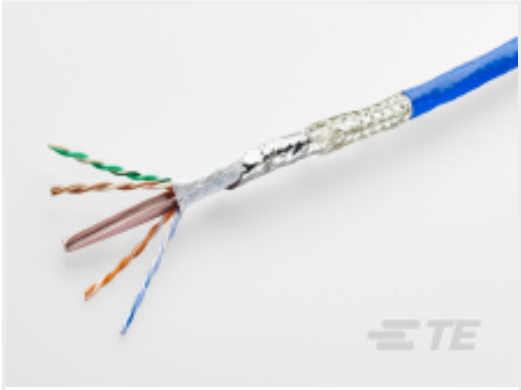
TE Part # EM3665-000 C6A-26C444X814-9
