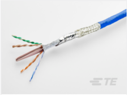
TE Part # EH2156-000 C6A-24C444-814-9
