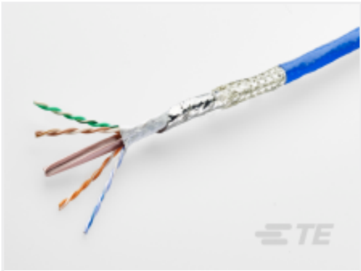
TE Part # CQ61803001 C6A-24B134XM18A-0CK9500
