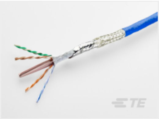
TE Part # CQ53593001 C6A-24B134XN1FA-0CK9500
