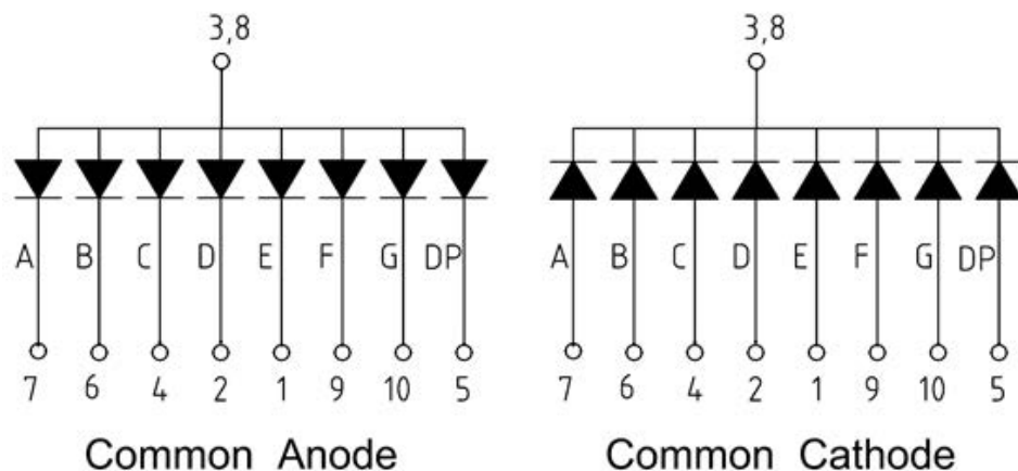
Figure 2: Circuit Diagram
