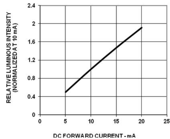
Figure 9: Relative Luminous Intensity vs. Forward Current
