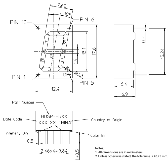
Figure 1: Package Dimension
