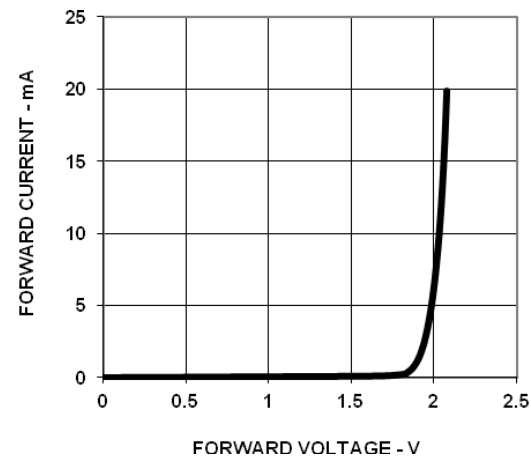
Figure 4: Forward Voltage vs. Current
