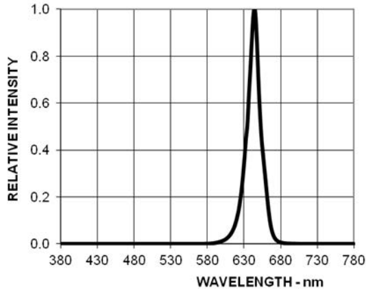
Figure 11: Relative Luminous intensity vs. Wavelength
