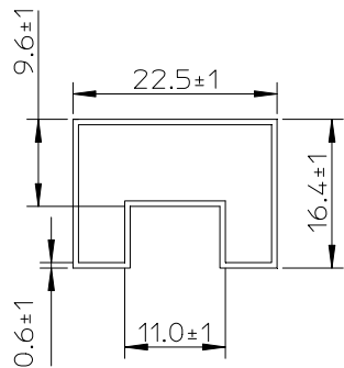
Tube Front View
