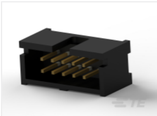
TE Part # 5103310-1 A/L LOW PRO HDR 10P RA BLACK
