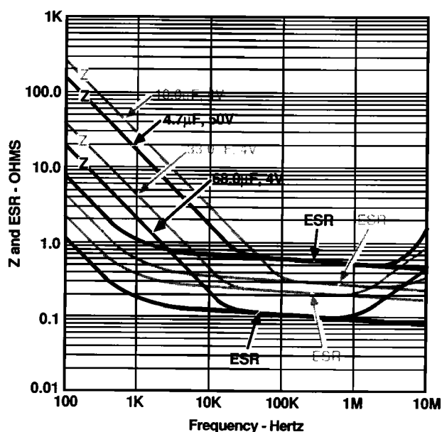
FIGURE 7c ESR & Impedance (Z) vs Frequency Typical T411/T421
