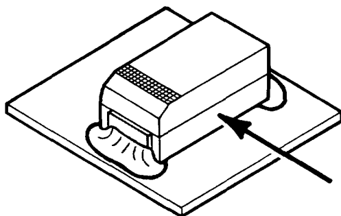
FIGURE 11 Shear Test
