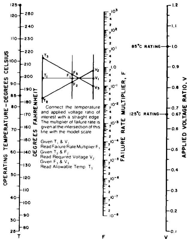
FIGURE 12 Reliability Nomograph
