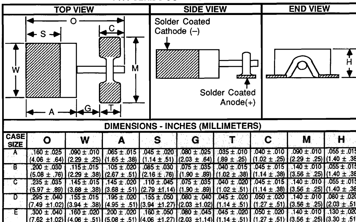
T411 SERIES OUTLINE DRAWINGS
