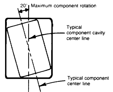
FIGURE 20 Component Rotation
