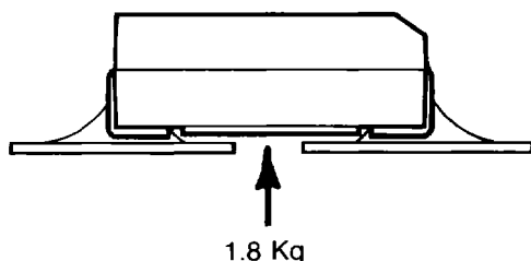
FIGURE 10 Tensile Test
