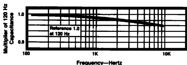
FIGURE 1 Typical Effect of Frequency upon Capacitance
