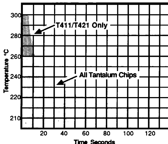
FIGURE 17 Time/Temperature Soldering Profile
