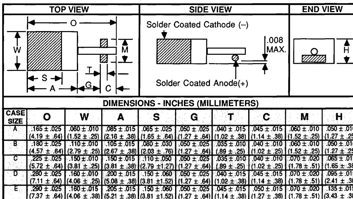
T421 SERIES OUTLINE DRAWINGS
