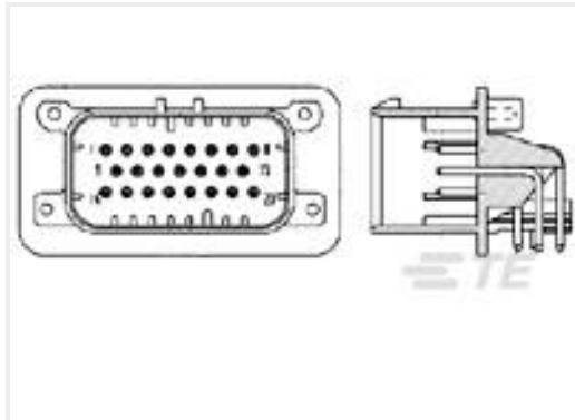
TE Part #776087-2 23POS,PIN DIA 1.3,HDR ASSY,90DEG, COD 2
