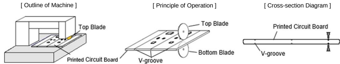
[ Disc Separator ]
