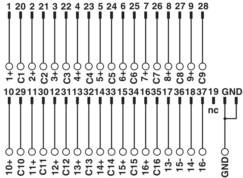
Connection scheme VIP-3/SC/D37SUB/M/HW/C300
