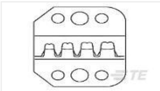
TE Part #58525-2 PROCrimper DIE
