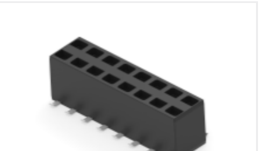
TE Part # 969973-8 2x8P HV100 REC. CON, SMD, GOLD, BLISTER
