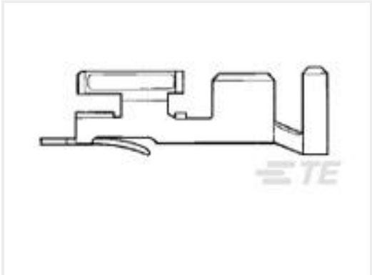
TE Part #350821-1 HERM HI/CUR TERM 12-8 LP
