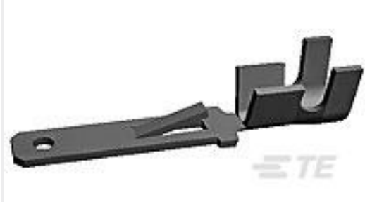
TE Part #928962-4 FF 250 TAB 17-13 AWG .016 TPBR
