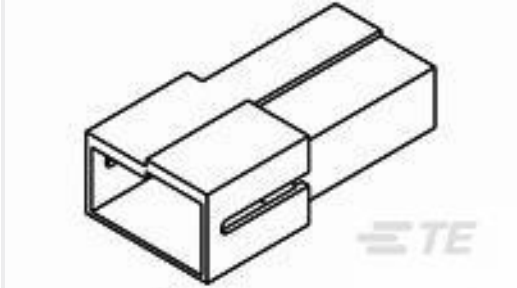
TE Part #626065 2 P FASTIN-ON 110 HOUSING TAB PA66 NAT
