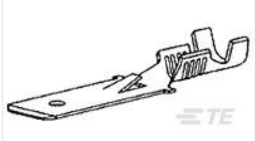
TE Part #160762-2 FF 110 TAB 0.5-1.5MM2 PTPBR
