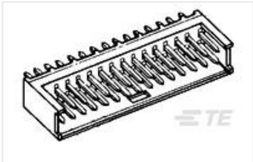
TE Part #280385-1 2X8P AMPMODU II SHRD HDR, ST, TIN
