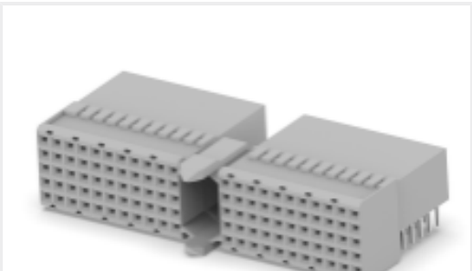
TE Part #3-5100147-0 Z-PACK,TYPE A, RA REC.110P
