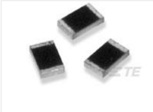
TE Part #4-1879267-7 RP 2B 976K 0.1% 15PPM 1K RL
